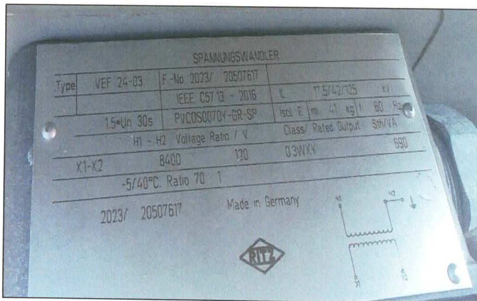
Item no. 14. Transformer, current transformer, outdoor, 400:5
